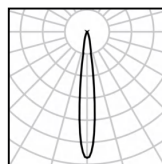
6W Ra98 3000K 15°
